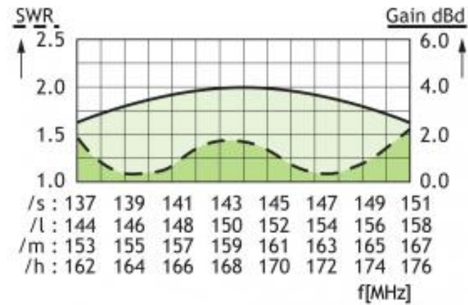
TYPICAL GAIN AND SWR CURVES
